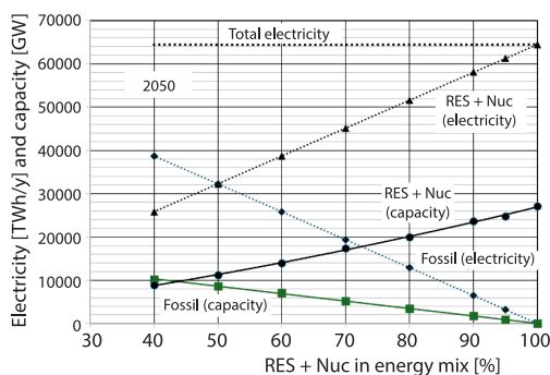
Figure 4. Electricity production and capacity of plants in 2050
