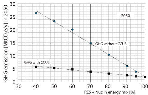
Figure 5. The GHG emissions with and without CCUS technologies
