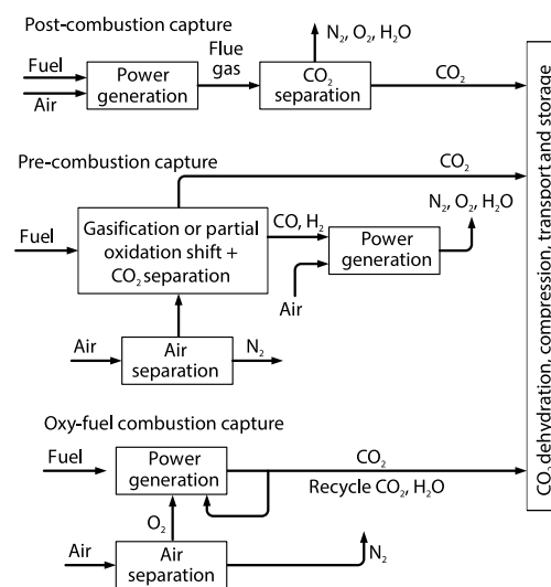
Figure 2. Post-combustion, pre-combustion, and oxy-fuel combustion capture technologies
