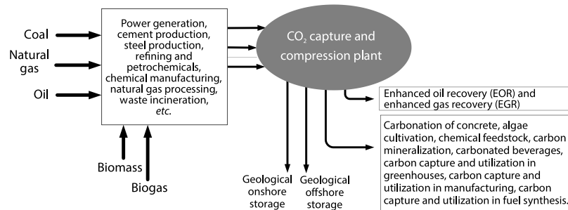
Figure 1. Conceptual role of the CCUS plant
