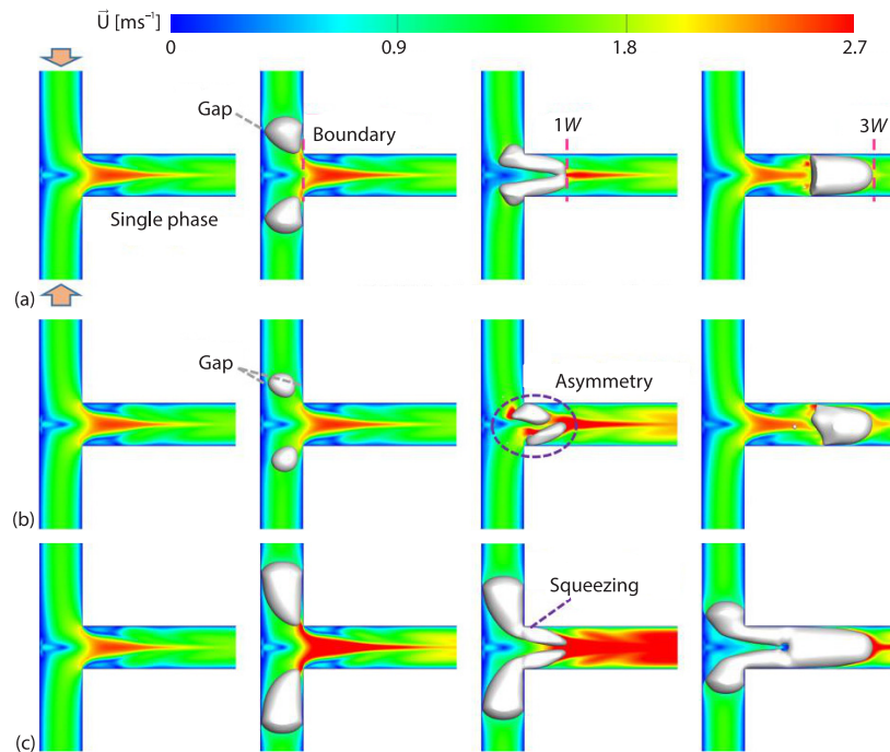
Figure 4. Bubble shapes and velocity fields during the merger process at different heat fluxes and seed bubble volumes; (a) q = 2000 \text{ W/m}^2 , D^* = 0.8 , (b) q = 8000 \text{ W/m}^2 , D^* = 0.6 , and (c) q = 8000 \text{ W/m}^2 , D^* = 0.8
