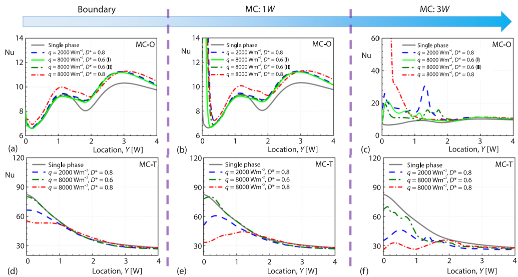
Figure 8. Distribution of Nusselt number for the downstream main channel
