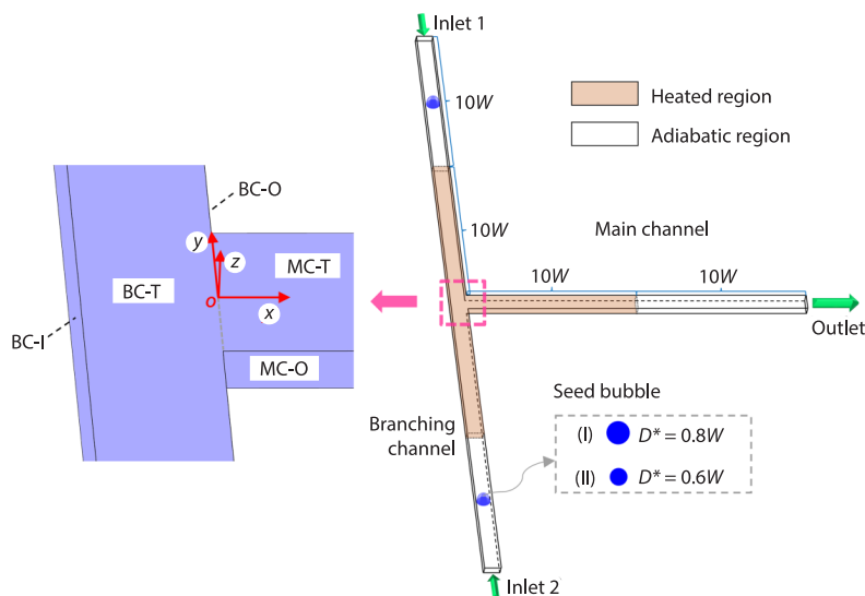
Figure 1. The diagrammatic sketch for bubble merger in heated symmetric micro-fluidic T-junction and the definition of various walls
