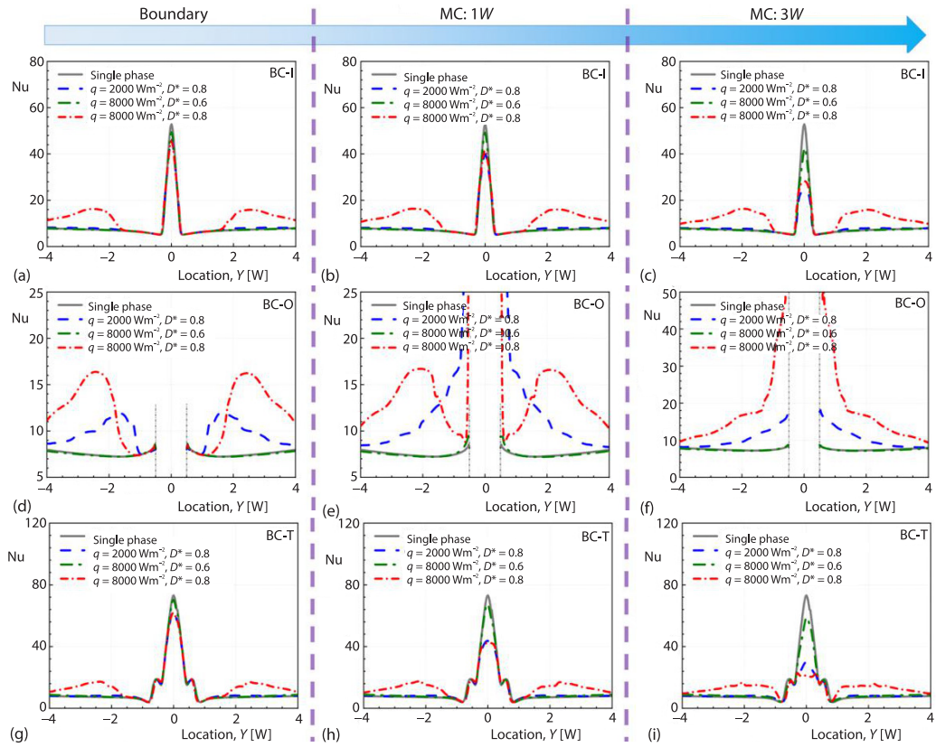
Figure 7. Distribution of Nusselt number for the upstream branching channel
