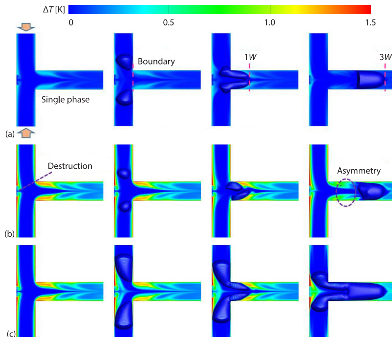
Figure 6. Temperature fields at different heat fluxes and seed bubble volumes; (a) q = 2000 \text{ W/m}^2 , D^* = 0.8 , (b) q = 8000 \text{ W/m}^2 , D^* = 0.6 , and (c) q = 8000 \text{ W/m}^2 , D^* = 0.8
