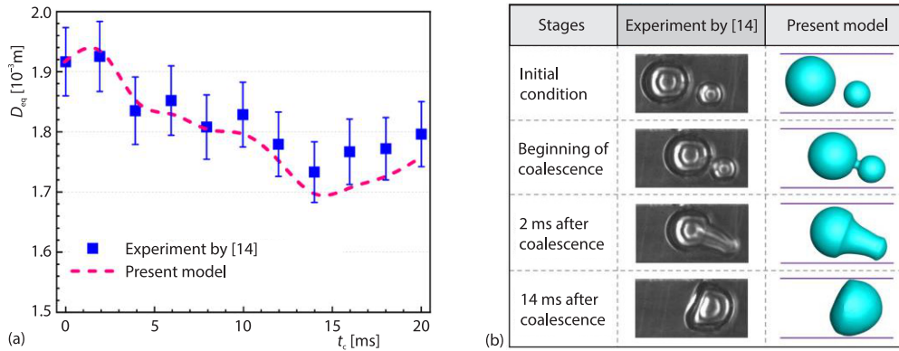
Figure 3. Validation of the developed numerical model by the experimental results from [14]; (a) equivalent bubble diameter and (b) bubble shape
