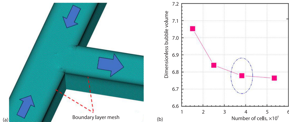
Figure 2. Mesh configuration (a) and independence test (b)
