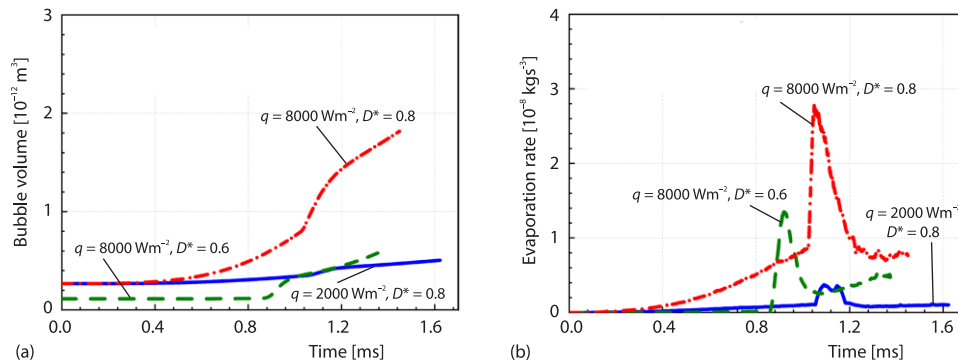
Figure 5. The evolutions of bubble volume and evaporation rate; (a) bubble volume and (b) evaporation rate
