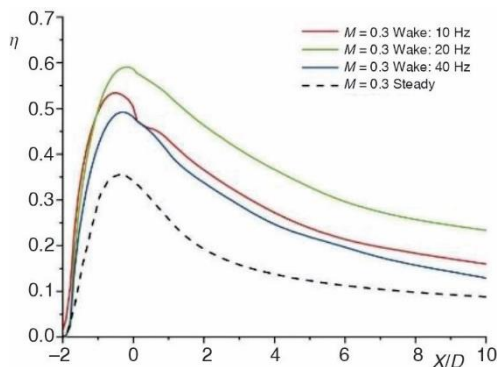
Figure 5. Streamwise distributions of laterally-averaged film cooling effectiveness
