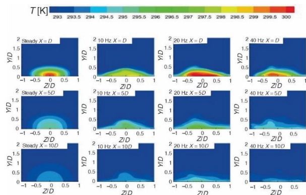
Figure 7. Contours of temperature at different streamwise locations
