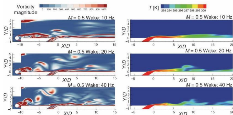
Figure 8. Instantaneous contours of vorticity and temperature in z = 0
