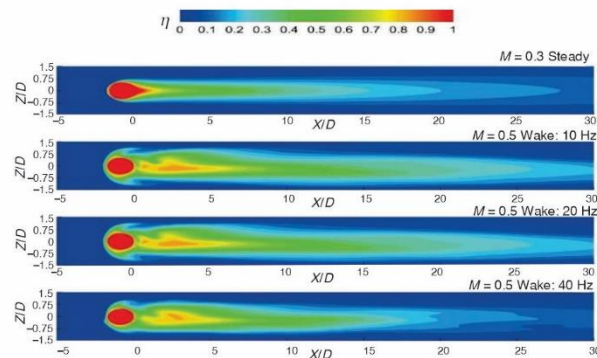
Figure 9. Contours of time-averaged film cooling effectiveness on the plate
