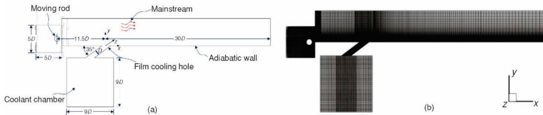
Figure 1. Schematic diagram of the computational domain and grid
