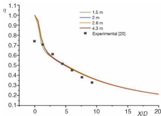
Figure 2. Streamwise distribution of the film cooling effectiveness with different grids
