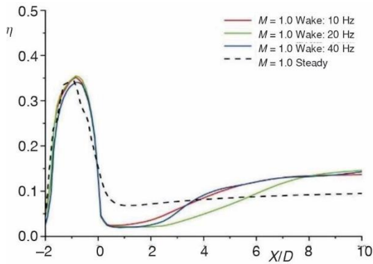
Figure 13. Streamwise distributions of laterally-averaged film cooling effectiveness
