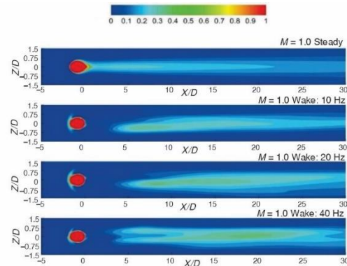
Figure 14. Contours of time-averaged film cooling effectiveness on the plate
