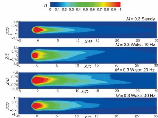
Figure 6. Contours of time-averaged film cooling effectiveness on the plate
