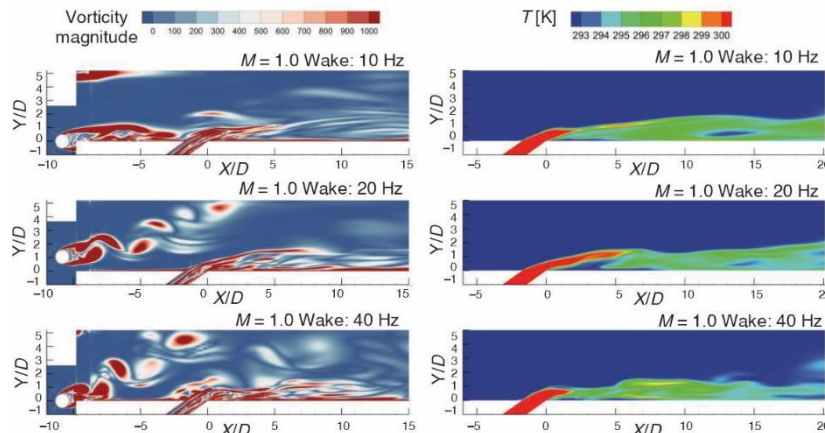
Figure 12. Instantaneous contours of vorticity and temperature in z = 0
