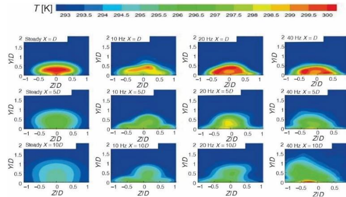
Figure 11. Contours of temperature at different streamwise locations
