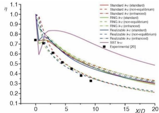
Figure 3. Streamwise distribution of the film cooling effectiveness with different turbulence models
