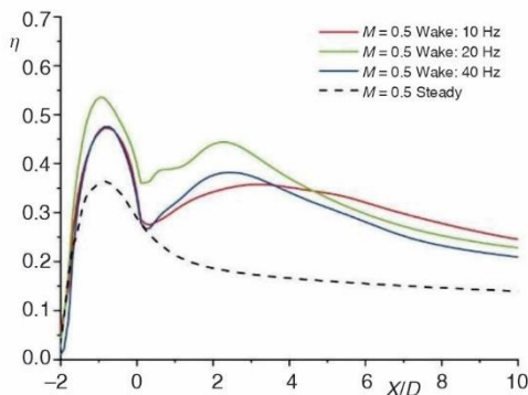
Figure 10. Streamwise distributions of laterally-averaged film cooling effectiveness
