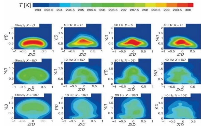
Figure 15. Contours of temperature at different streamwise locations
