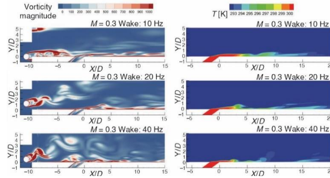
Figure 4. Instantaneous contours of vorticity and temperature in z = 0
