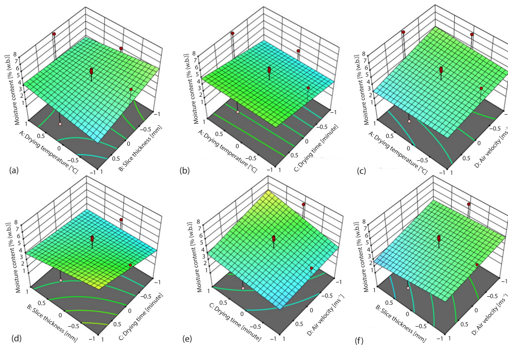
Figure 4. Plots of response surface for dependent variable (MC) while drying ivy gourd
