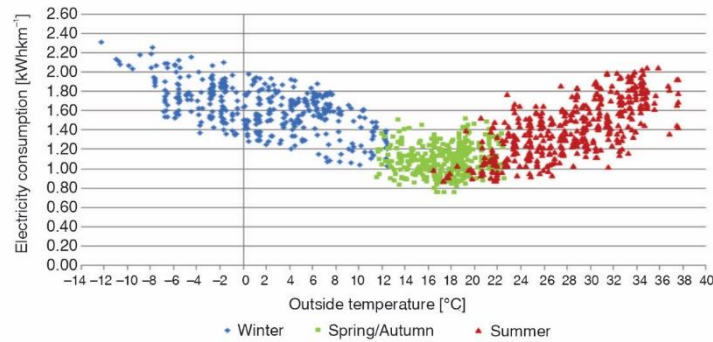
Figure 5. Electricity consumption and outside temperature, line EKO1, direction A, winter, transition, summer period
