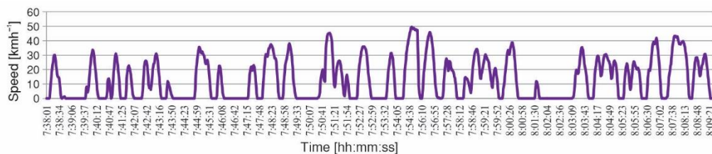
Figure 2. Driving cycle on the line EKO1, direction A, period 7:38:01 to 8:09:30
