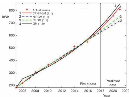
Figure 5. Trend of per capita electricity consumption for daily life in China
