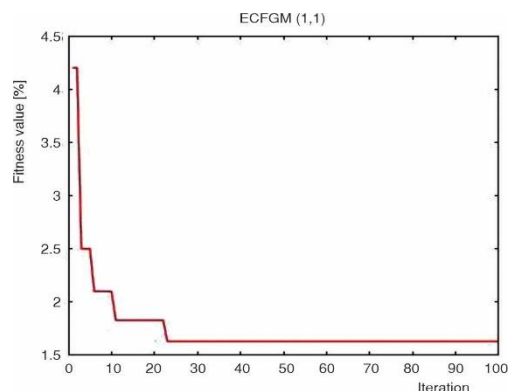
Figure 3. Track of searching for the optimal power index by PSO
