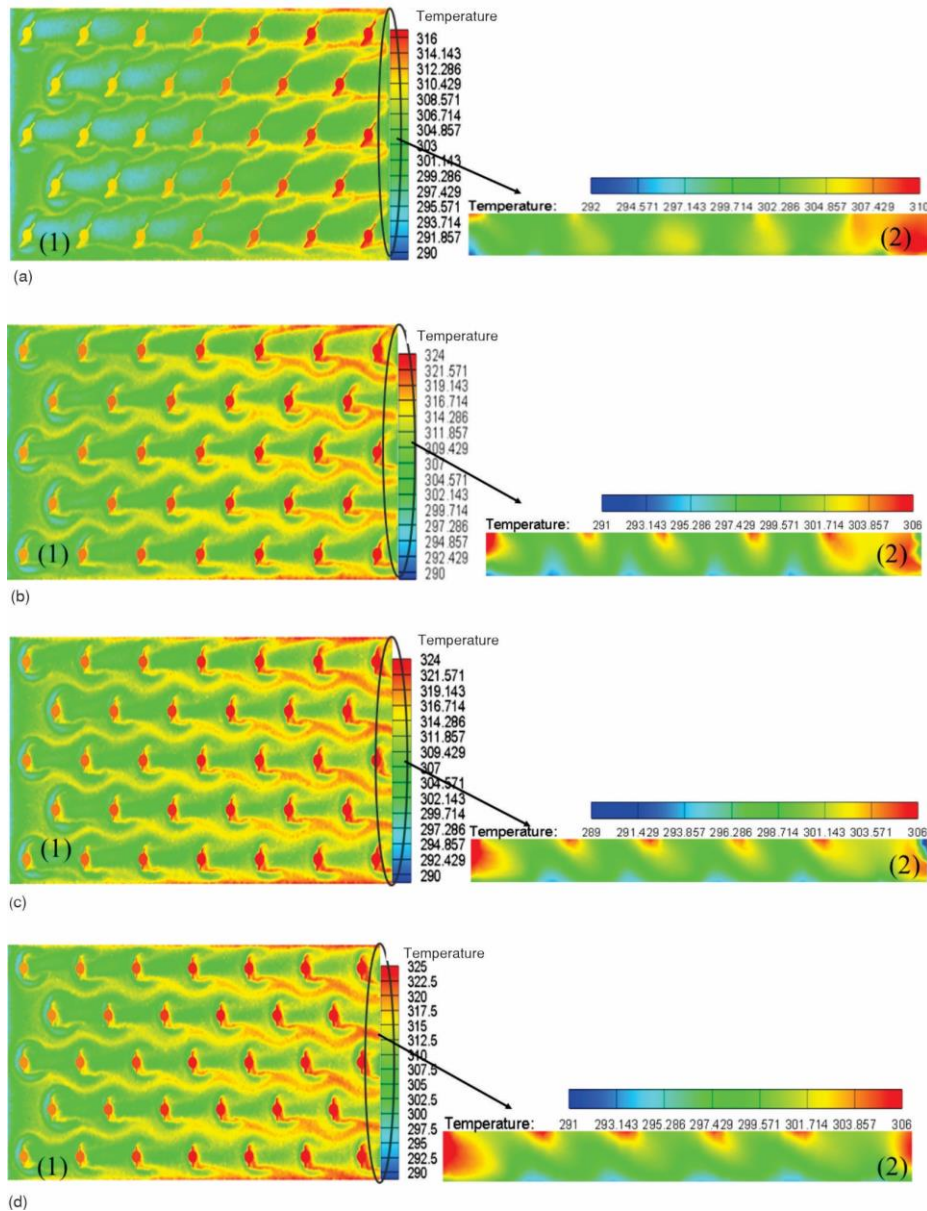
Figure 8. The temperature distribution of the collector with fins of different guide vane pitches; (a) temperature distribution of the collector with guide vane pitches of 160 mm, (b) temperature distribution of the collector with guide vane pitches of 210 mm (c) temperature distribution of the collector with guide vane pitches of 260 mm, and (d) temperature distribution of the collector with guide vane pitches of 310 mm
