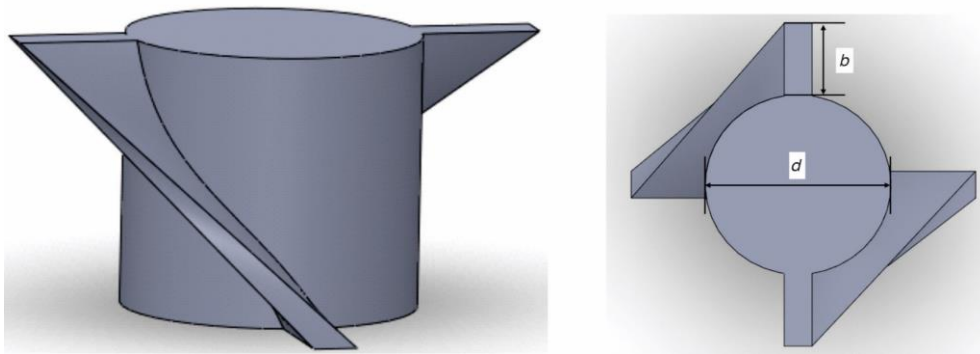
Figure 2. Structure of fins
