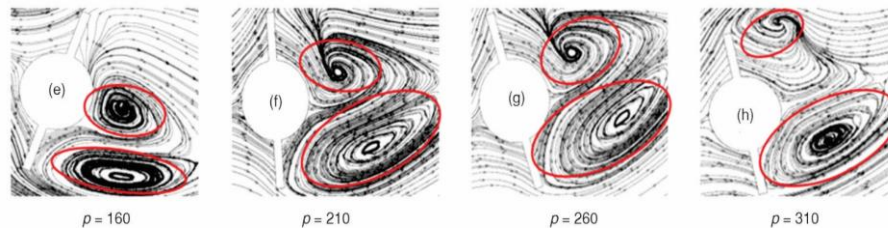
Figure 9. The internal air streamline diagram of the collector under different pitches of the deflectors
