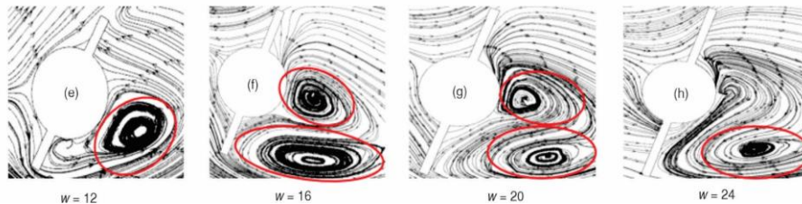
Figure 6. The internal air streamline diagram of the collector under different widths of the deflectors
