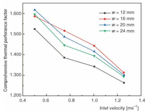
Figure 7. Changes of comprehensive performance factors of collectors at different flow rates
