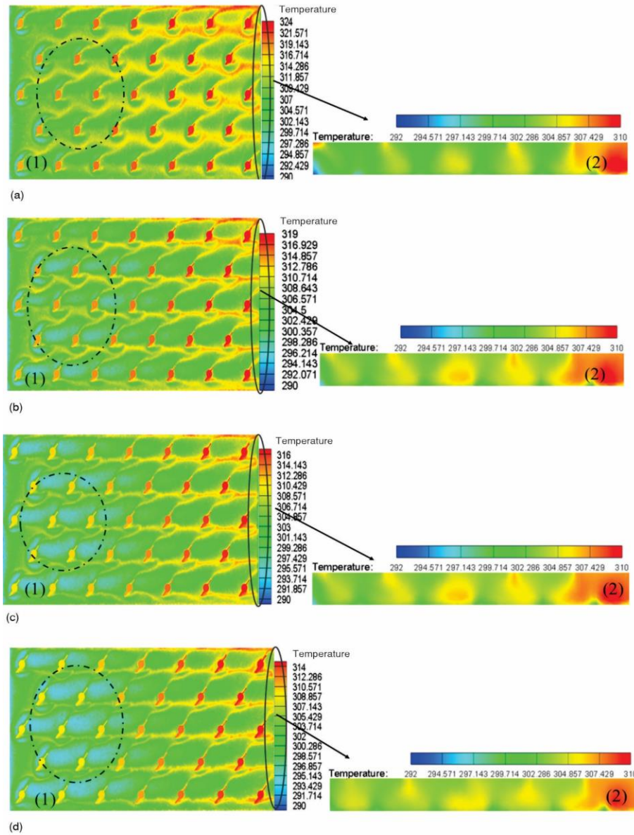
Figure 5. The temperature distribution of the collector with fins of deflector widths; (a) temperature distribution of the collector with deflector widths of 12 mm, (b) temperature distribution of the collector with deflector widths of 16 mm, (c) temperature distribution of the collector with deflector widths of 20 mm, and (d) temperature distribution of the collector with deflector widths of 24 mm
