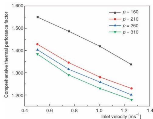
Figure 10. The change of CTPF of collector under different inlet flow rates
