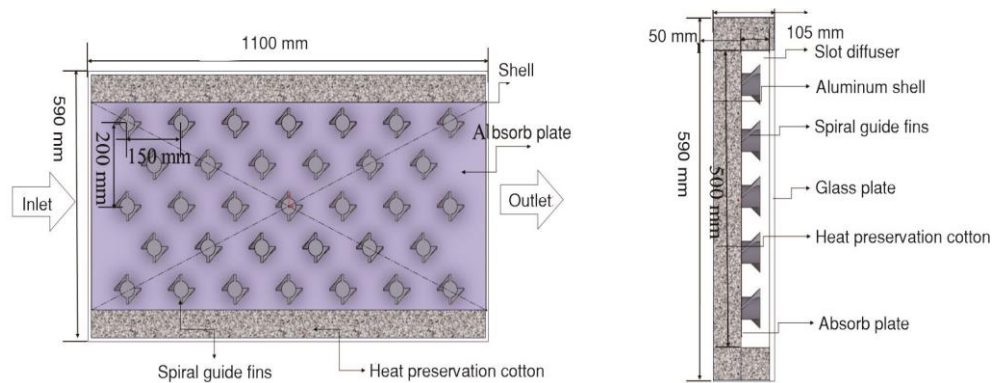
Figure 1. Main view of structure design of spiral finned plate collector
