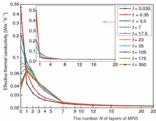
Figure 10. The influence of N on the thermal insulation performance
