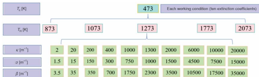
Figure 2. Calculation condition of the computational domain without MRS
