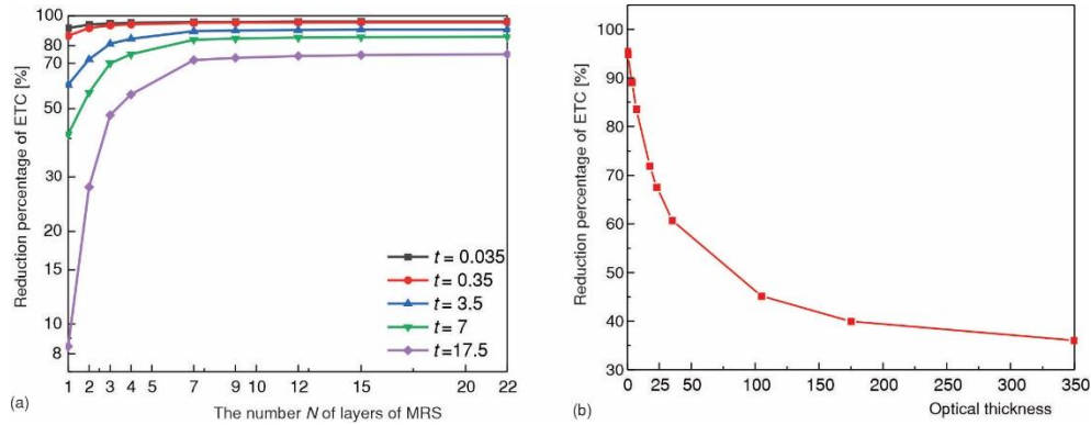
Figure 11. Reduction percentage of ETC; (a) different N compared to no MRS and (b) seven layers of MRS compared to no MRS
