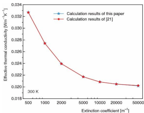
Figure 7. Validation of numerical method
