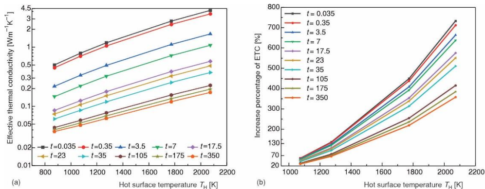
Figure 8. The variation of ETC; (a) variation of ETC at different T_H and (b) increase percentage of ETC at different T_H
