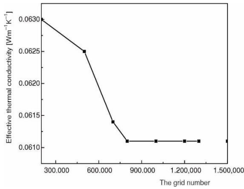
Figure 6. The variation of ETC with the number of grids
