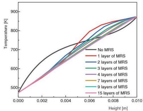
Figure 12. Temperature curve along z -axis direction at center of semi-transparent material
