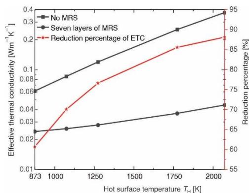
Figure 13. Reduction percentage of ETC of materials with seven layers of MRS at different T_H
