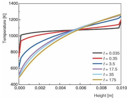
Figure 9. Temperature curve along z -axis direction at boundary of semi-transparent materials
