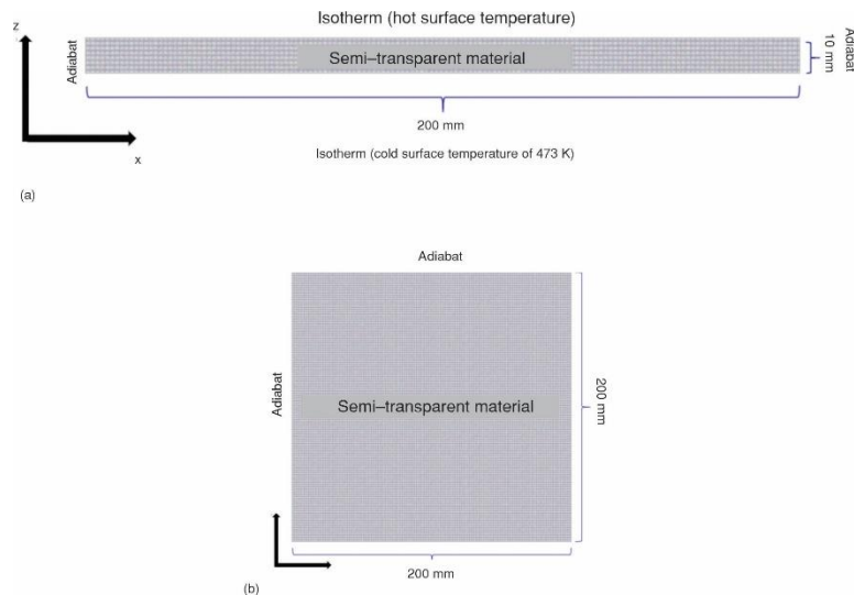
Figure 1. The computational domain; (a) front view and (b) top view
