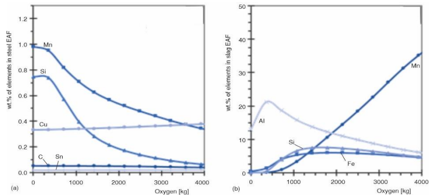
Figure 9. Distribution of elements per oxygen input in; (a) Steel EAF and (b) slag EAF at 1600 °C
