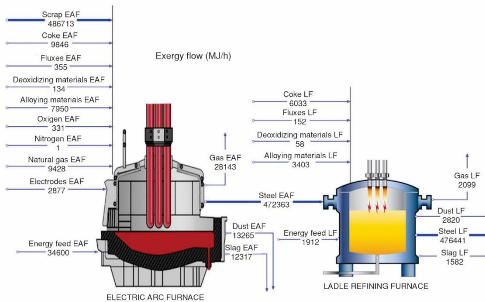
Figure 4. Exergy flow for EAF and LF
