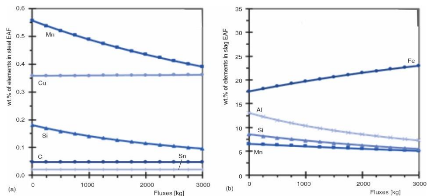
Figure 11. Distribution of elements per fluxes input in; (a) Steel EAF and (b) slag EAF at 1600 °C
