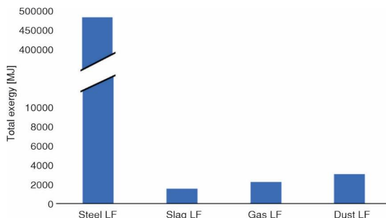
Figure 8. Total exergy of output materials of LF
