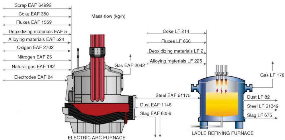
Figure S1. Mass-flow for EAF and LF
