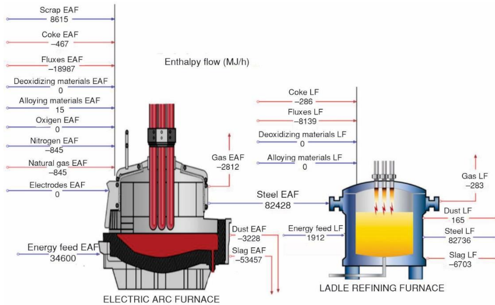
Figure 3. Enthalpy flow for EAF and LF
