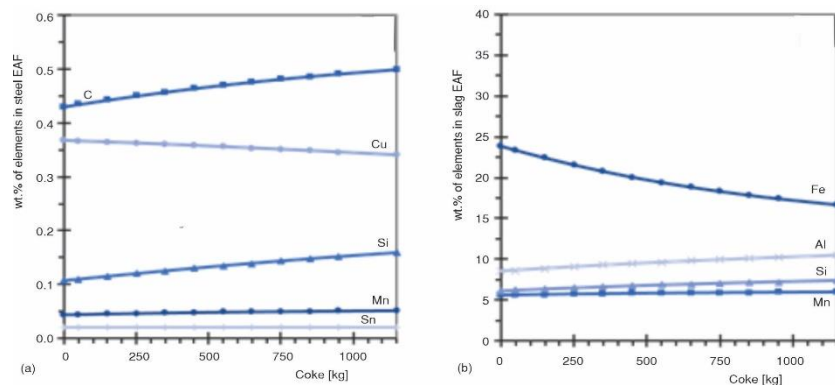
Figure 10. Distribution of elements per coke input in; (a) Steel EAF and (b) slag EAF at 1600 °C
