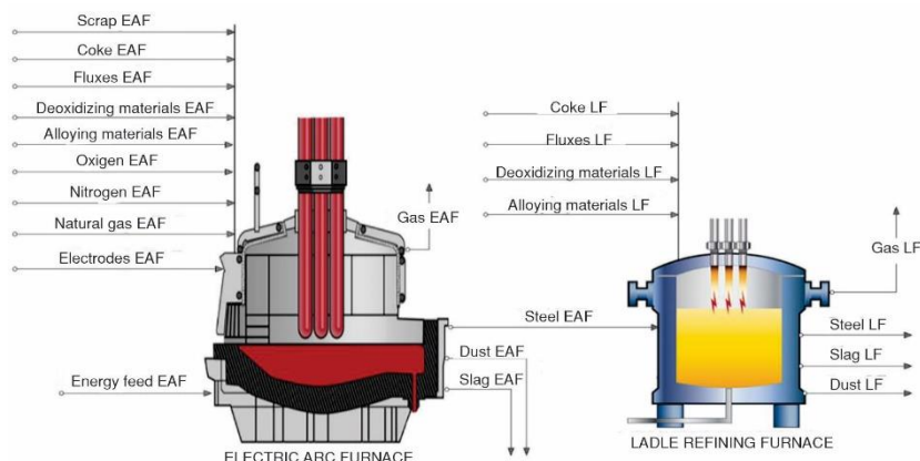
Figure 1. Setting up material flows in an EAF and ladle furnace (LF)
