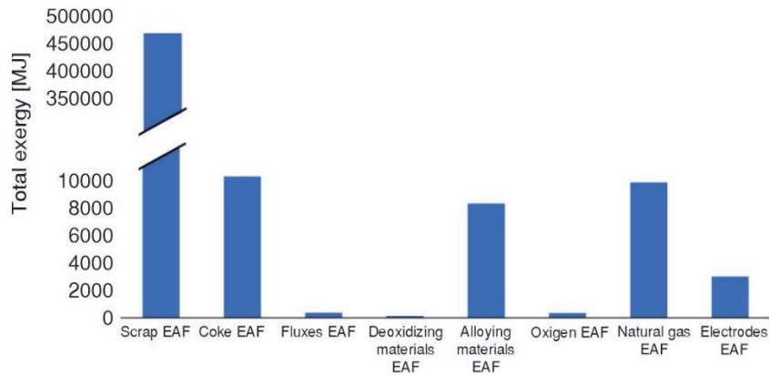
Figure 5. Total exergy of input materials of EAF
