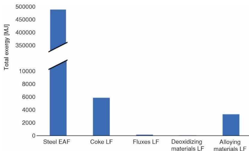
Figure 7. Total exergy of input materials of LF
