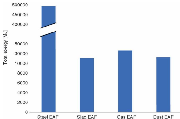
Figure 6. Total exergy of output materials of EAF
