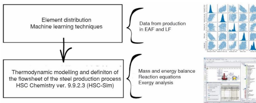
Figure 2. Modeling procedure for performing the exergy analysis
