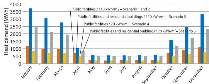
Figure 1. Overview of the heat demand in different scenarios
