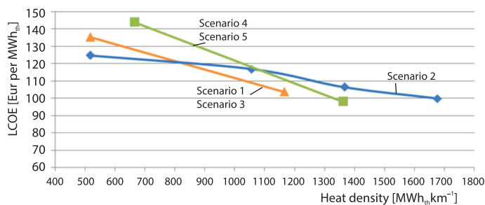
Figure 3. Impact of the linear heat density on the LCOE
