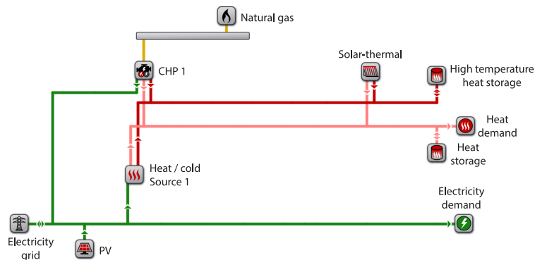
Figure 2. Scheme of the energy hub
