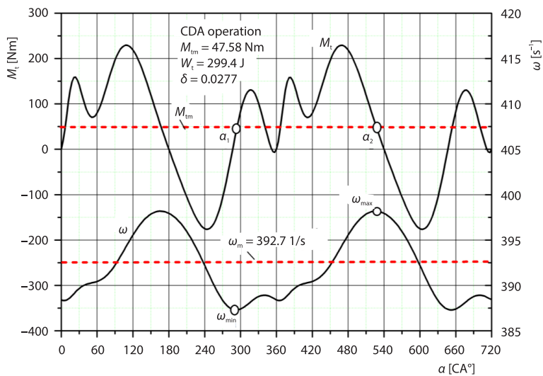
Figure 14. The variations of engine torque, M_t , and rotational speed, \omega ; CDA engine operation; 2 and 3 cylinders deactivated; n = 3750 rpm, BMEP = 4.362 bar
