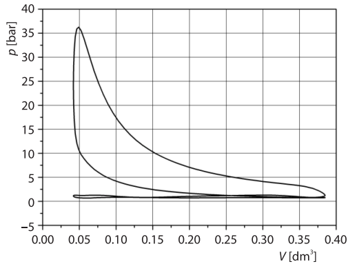
Figure 10. Indicator p - V diagram; n = 1800 rpm, BMEP = 2.62 bar; CDA engine operation, active cylinder 1, IMEP = 7.28 bar
