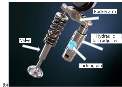
Figure 2. Mazda CDA system [8]
