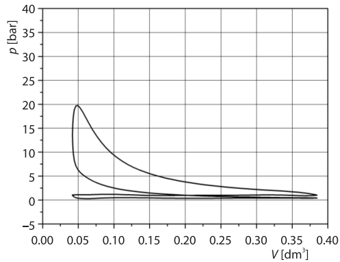
Figure 9. Indicator p - V diagram; n = 1800 rpm, BMEP = 2.62 bar; standard engine operation, cylinder 1, IMEP = 3.55 bar
