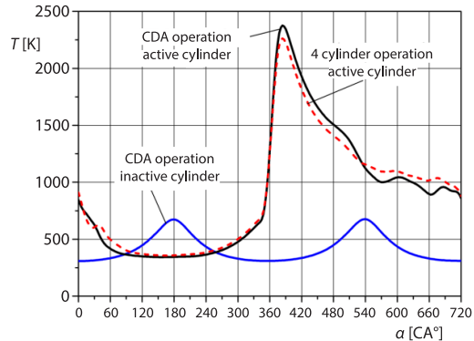
Figure 8. Temperatures vs. CA for engine standard and CDA operation; n = 1800 rpm, BMEP = 2.62 bar
