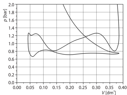
Figure 12. Low pressure part of indicator p - V diagram (pumping work); CDA engine operation; active cylinder 1; n = 1800 rpm, BMEP = 2.62 bar, PMEP = -0.308 bar
