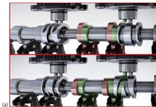
Figure 1. The VW CDA system [2]
