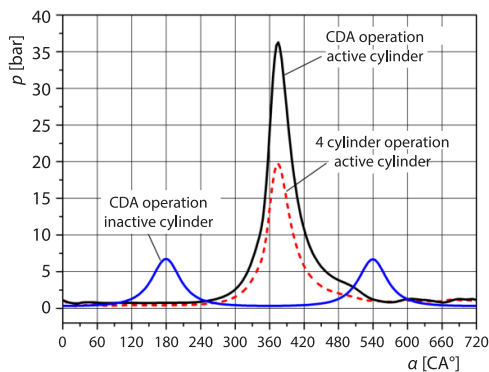
Figure 7. Pressures vs. CA for engine standard and CDA operation; n = 1800 rpm, BMEP = 2.62 bar
