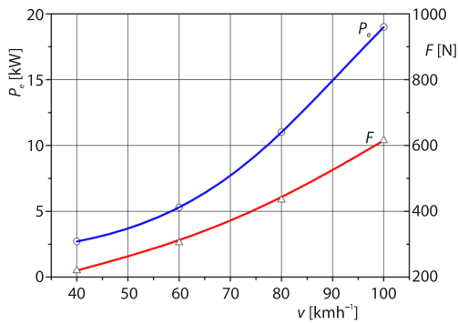
Figure 4. Vehicle tractive resistance force, F , and corresponding engine power, P_e
