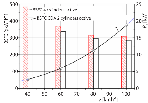
Figure 6. Required engine power, P_e , and BSFC
