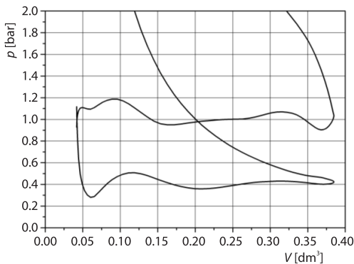
Figure 11. Low pressure part of indicator p - V diagram (pumping work); standard engine operation; cylinder 1; n = 1800 rpm, BMEP = 2.62 bar, PMEP = -0.601 bar
