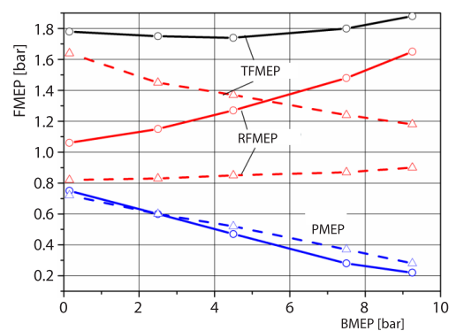
Figure 5. Mean effective pressure of losses vs. engine load; BMEP, PMEP, RFMEP, TFMEP – total friction mean effective pressure (PMEP + RFMEP + AMEP); full lines are for firing condition and dashed lines for motoring conditions; 4-cylinder 3.26 dm 3 spark ignition engine, n = 1600 rpm [16]
