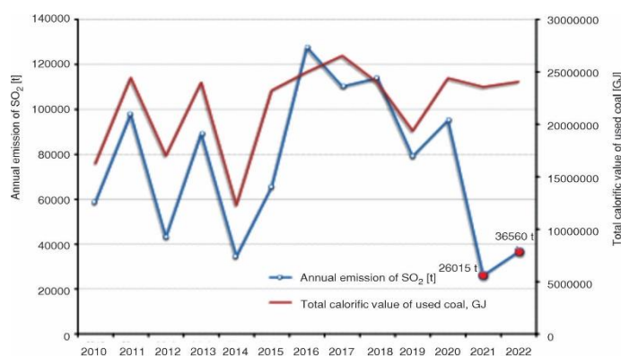
Figure 3. The dependence between the annual SO 2 emissions and the total calorific value of coal consumed in the TPP Kostolac B
