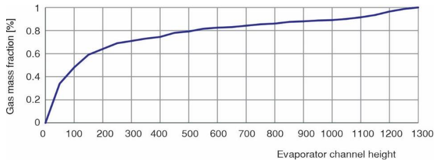
Figure 15. Gas mass fraction change
