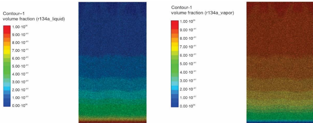
Figure 14. Display of liquid and gas volume fraction nephogram of refrigerant R134a in evaporator
