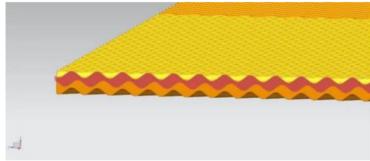
Figure 6. Partial model diagram of the plate side of the plate heat exchanger
