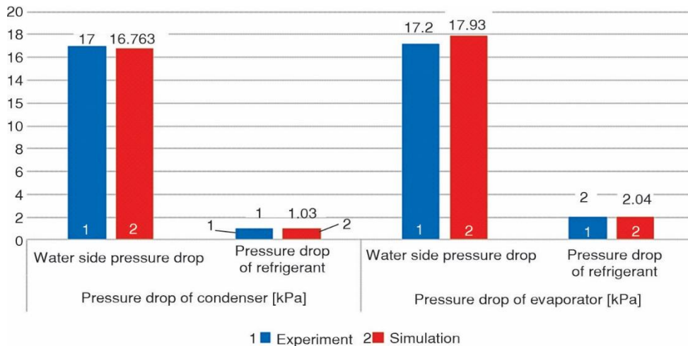
Figure 9. Comparison of experimental and simulated pressure drop results of condenser and evaporator
