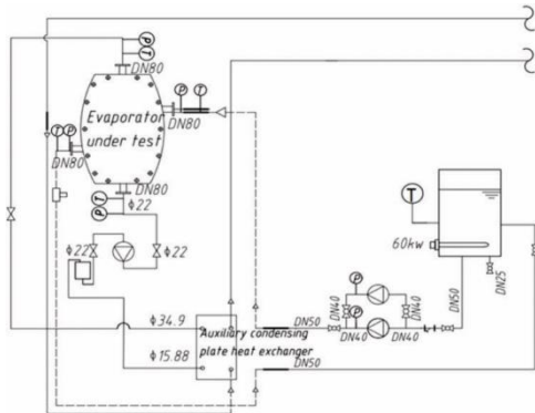
Figure 3. Experimental system diagram of evaporator
