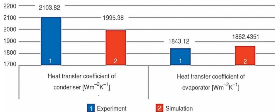
Figure 8. Comparison between experimental and simulation results of heat transfer coefficients results of evaporator and condenser
