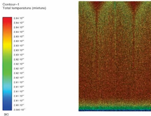
Figure 10. Display of temperature field cloud diagram of refrigerant side section of condenser
