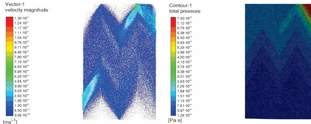
Figure 16. Display of velocity field and pressure field cloud map of evaporator water side section
