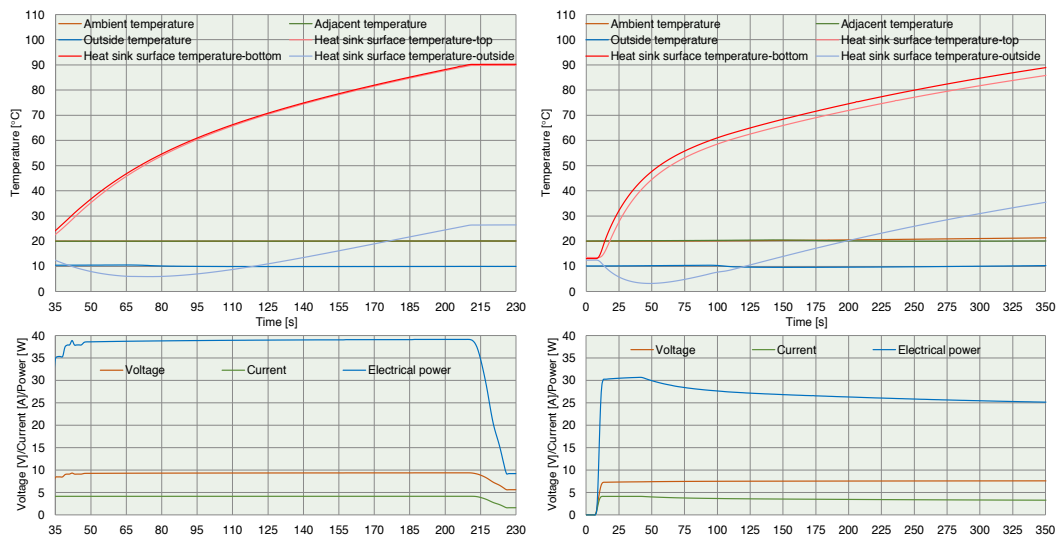
Figure 9. Experimental results of measurements of rapid heating of the aluminium heat exchanger; (a) a heat exchanger with non-optimal fin spacing and (b) a heat exchanger with optimal fin spacing
