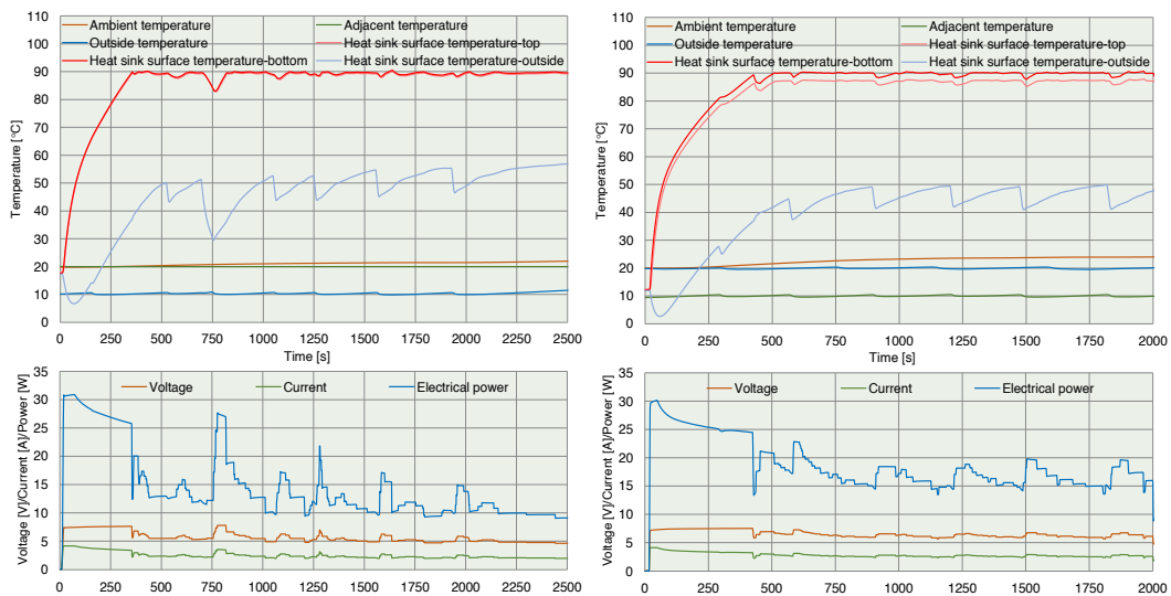
Figure 11. Experimental results of measuring regulated heating of the heat exchanger; (a) a heat exchanger with non optimal fin spacing and (b) a heat exchanger with optimal fin spacing
