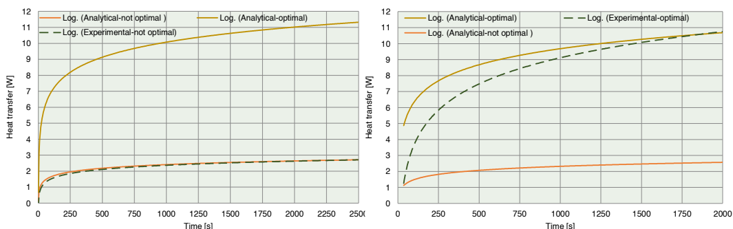
Figure 12. The comparison of analytical and experimental results of measurements shown in fig. 9; (a) a heat exchanger with non-optimal fin spacing and (b) a heat exchanger with optimal fin spacing
