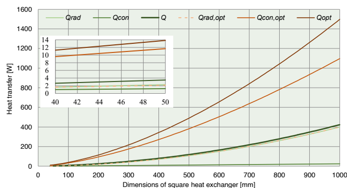
Figure 7. Heat transfer for different heat exchanger dimensions at 90 °C
