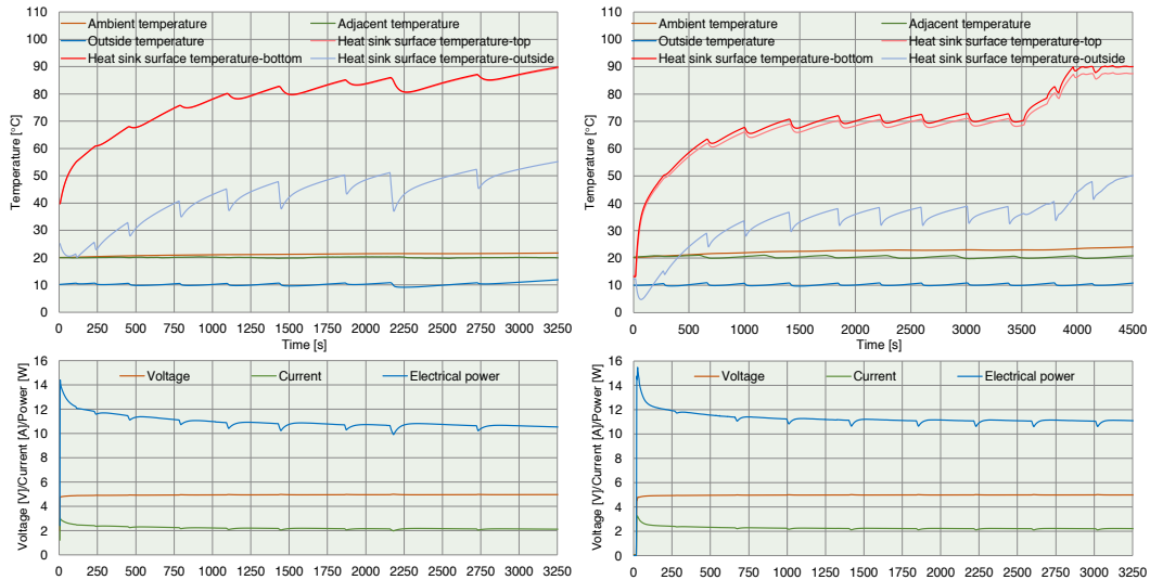
Figure 10. Experimental results of measuring gradual heating of the heat exchanger; (a) a heat exchanger with non-optimal fin spacing and (b) a heat exchanger with optimal fin spacing
