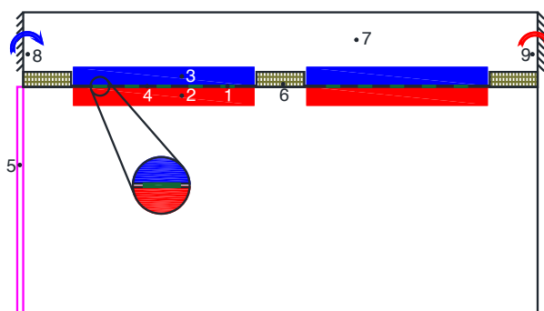
Figure 2. Heating system with TEM positioned in the ceiling; 1 – thermoelectric module, 2 – heat sink-hot side, 3 – heat sink-cold side, 4 – module carrier-plexiglas, 5 – PV module, 6 – insulation, 7 – air duct, 8 – air inlet, and 9 – air outlet
