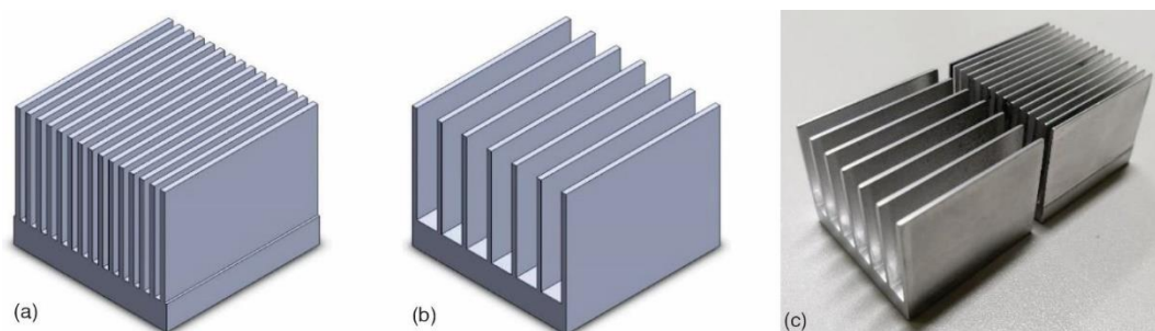
Figure 4. Heat exchangers for the heating system; (a) a heat exchanger model with non-optimal fin spacing; (b) a heat exchanger model with optimal fin spacing, and (c) a comparison of heat exchangers made with and without optimal fin spacing
