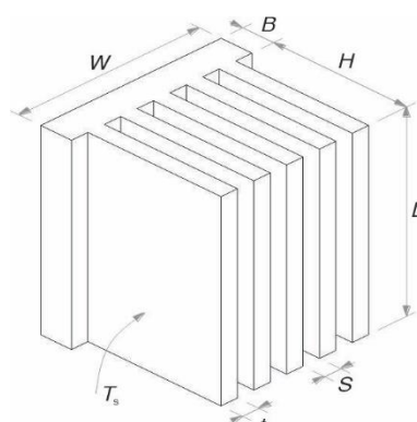
Figure 3. Dimensions of a finned surface oriented vertically
