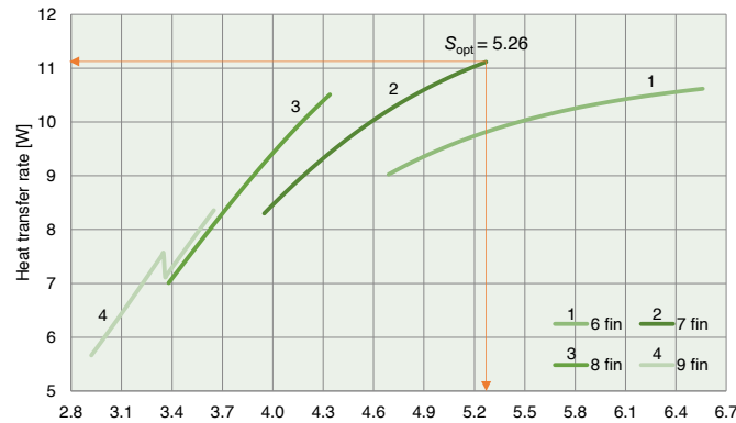
Figure 5. Optimum fin spacing for a 40×40 mm heat exchanger
