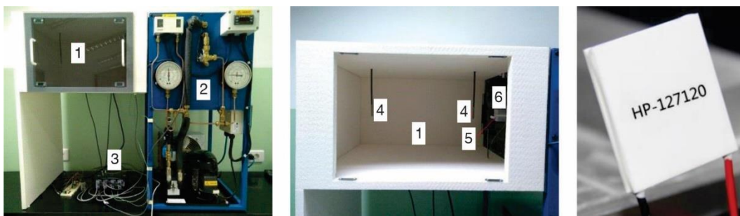
Figure 8. Experimental installation for the TEM analysis and Peltier module:
