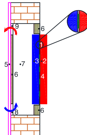
Figure 1. Heating system with TEM positioned in the wall; 1 – thermoelectric module, 2 – heat sink-hot side, 3 – heat sink-cold side, 4 – module carrier-plexiglas, 5 – PV module, 6 – insulation, 7 – air duct, 8 – air inlet, and 9 – air outlet
