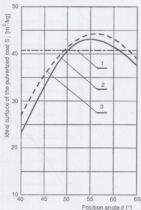
Figure 8. Dependence of the ideal surface of the pulverized coal from the obstacle cross-section and the position angle
